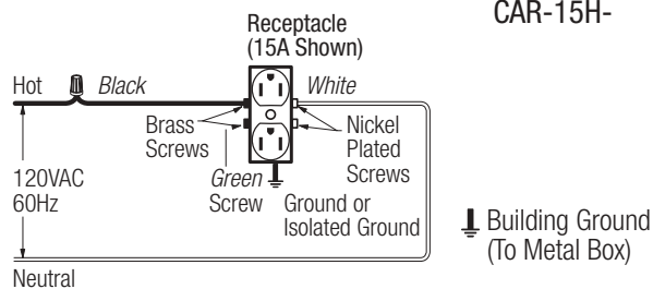
Wiring Diagram 7 Receptacle Wiring
