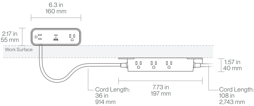
Charging Station Flat Mount - Front
