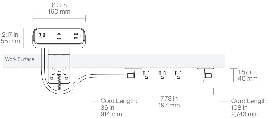
Charging Station Clamp Mount - Front
