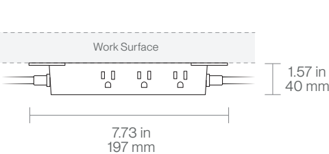
Main Power Brick - Back
