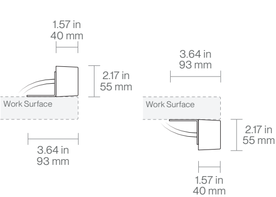
Charging Station Flat Mount - Side
