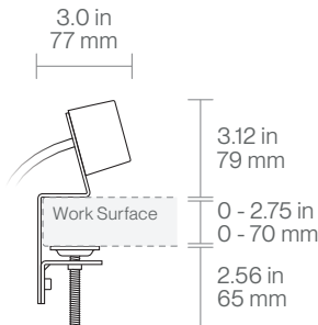
Charging Station Clamp Mount - Side
