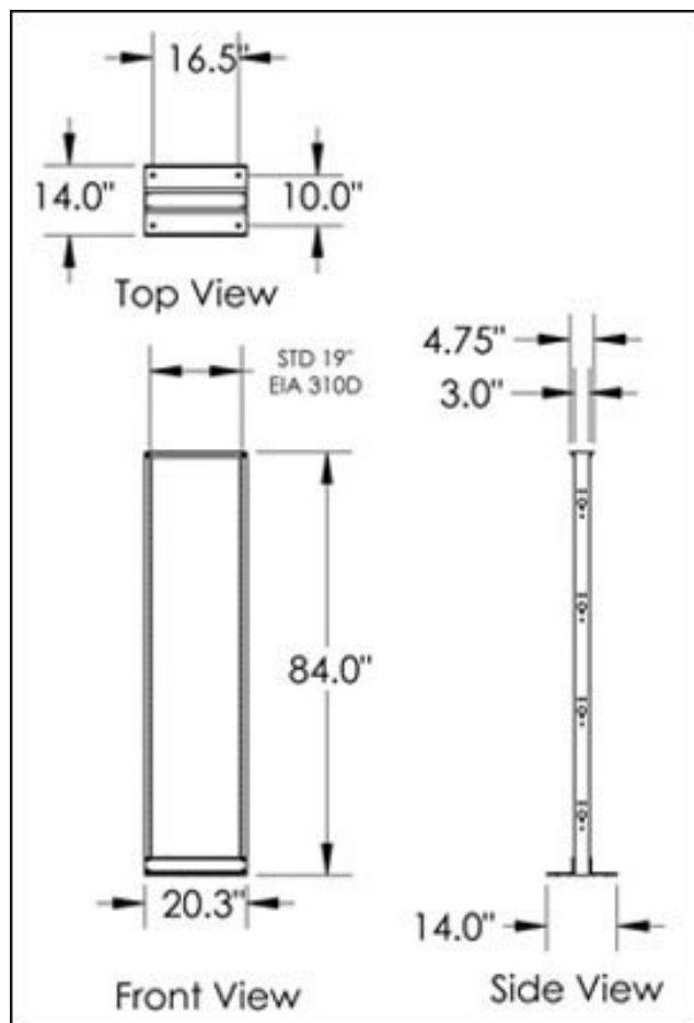
2-Post SmartRack Open Frame Rack Dimensions
