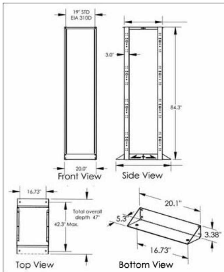
4-Post SmartRack Open Frame Rack Dimensions
