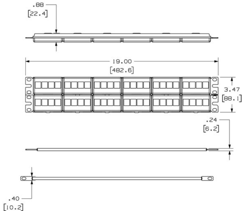
NetKey™ 48-Port Patch Panel w/ Strain Relief
