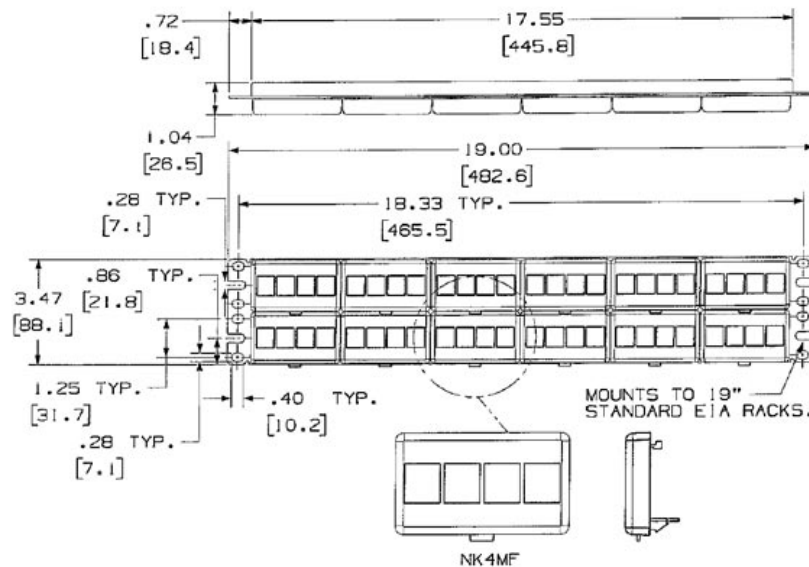
48-Port Patch Panel w/ Removable Faceplates
