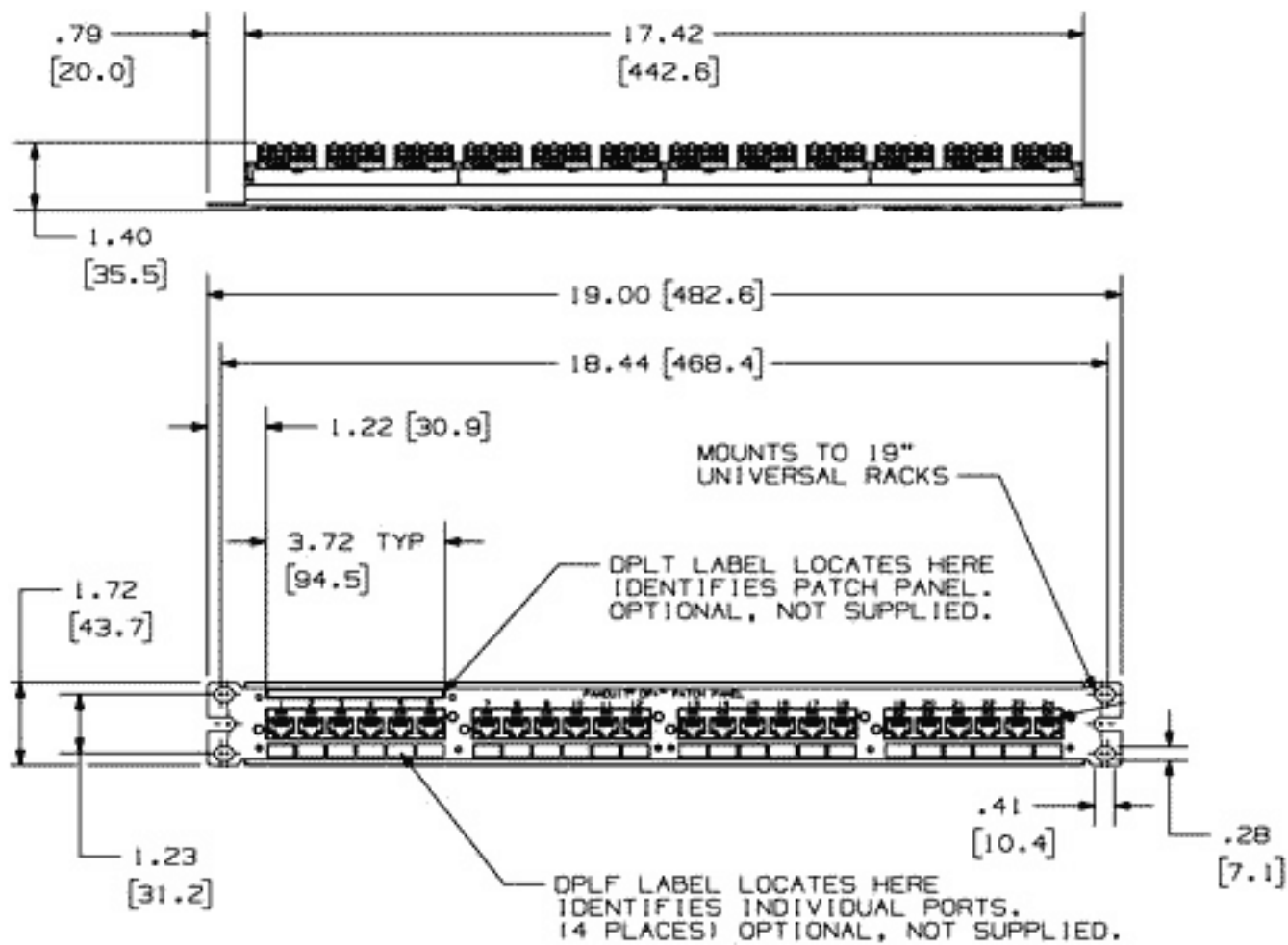
CAT5e 24 Port Patch Panel ITPAN-DP245E88TGY
