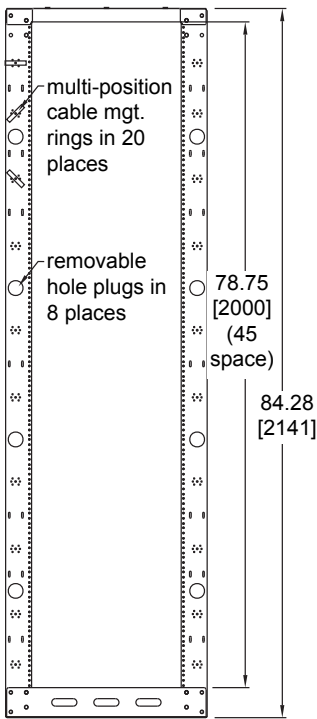
FRONT VIEW
