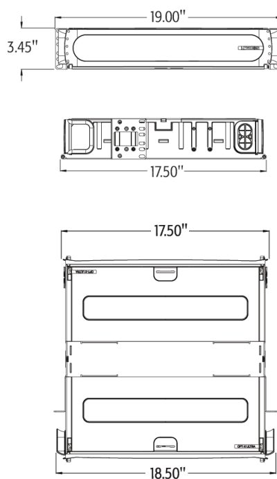
5R2UH-S06 (2RU)
