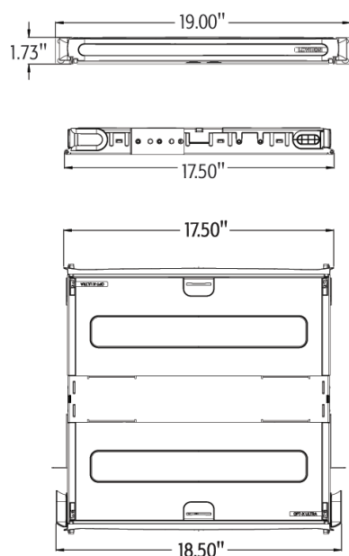
5R1UH-S03 (1RU)
