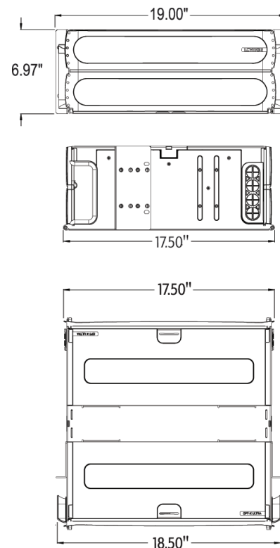
5R4UH-S12 (4RU)
