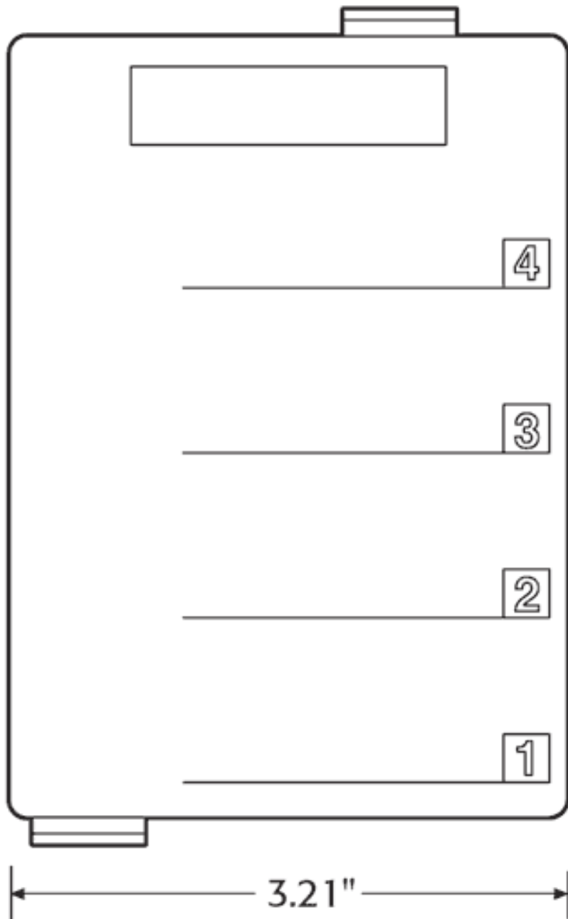
4 Port Surface Mount Housing 4.77" H x 3.21" W x 1.05" D
