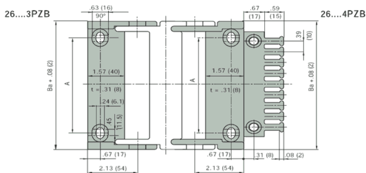
Pivoting Bracket Dimensions
