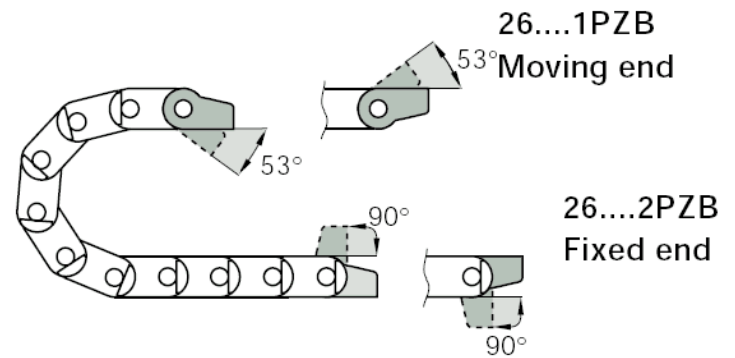
Pivoting Bracket Angles
