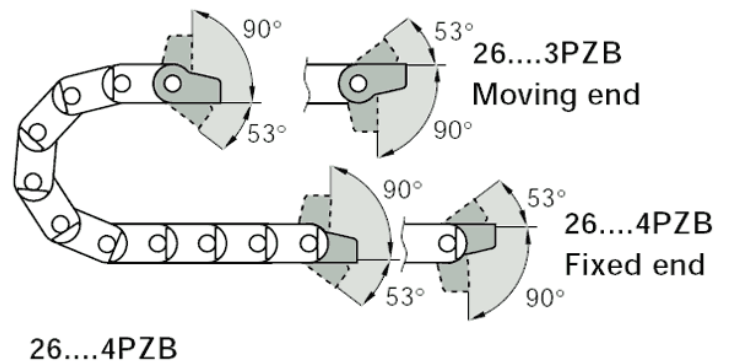
Pivoting Bracket Angles
