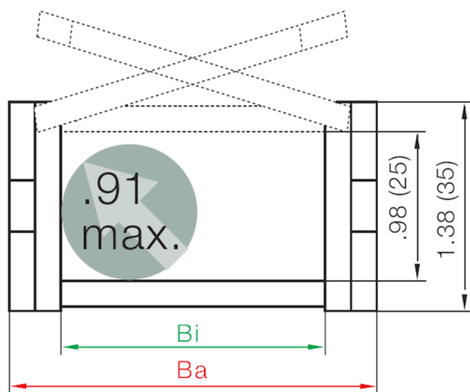
Series 250 - Snap-Open Along Outer Radius
