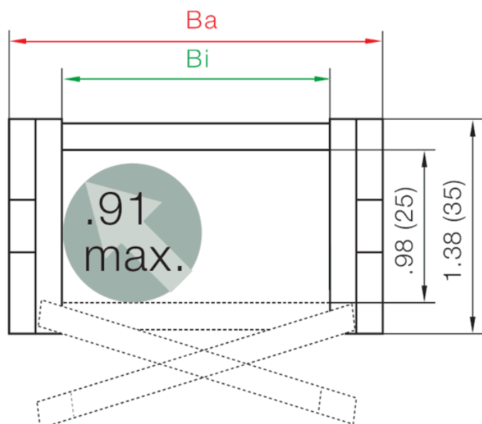
Series 240 - Snap-Open Along Inner Radius
