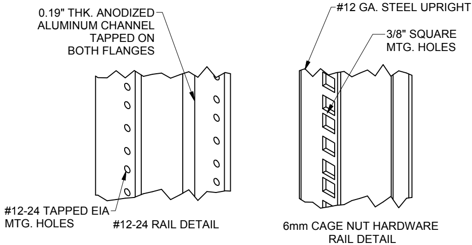
M6 OR #12-24 RAIL OPTIONS
