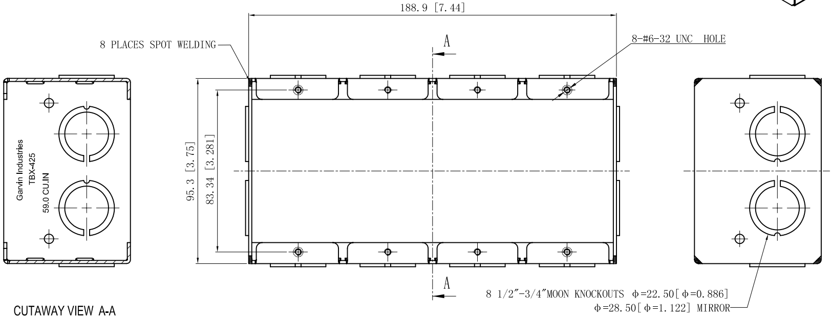
CUTAWAY VIEW A-A
