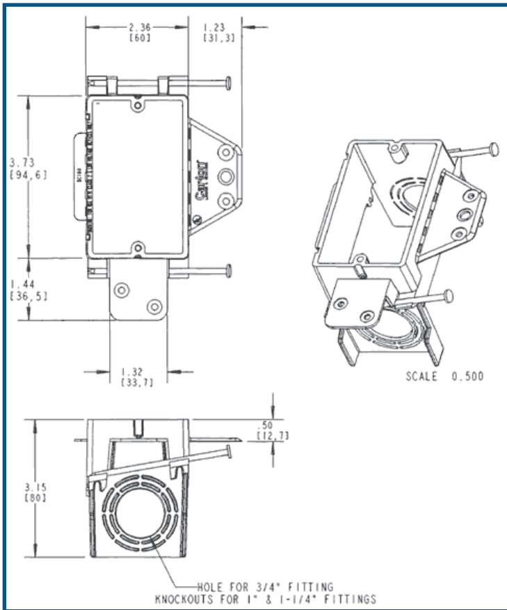
1-GANG NEW CONSTRUCTION
