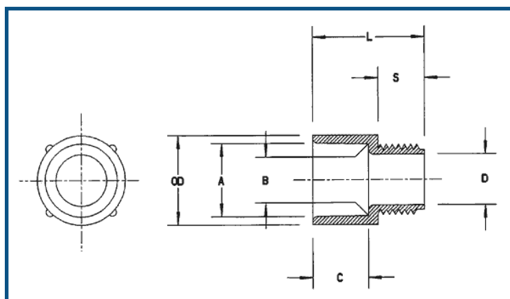
MALE TERMINATOR ADAPTER
