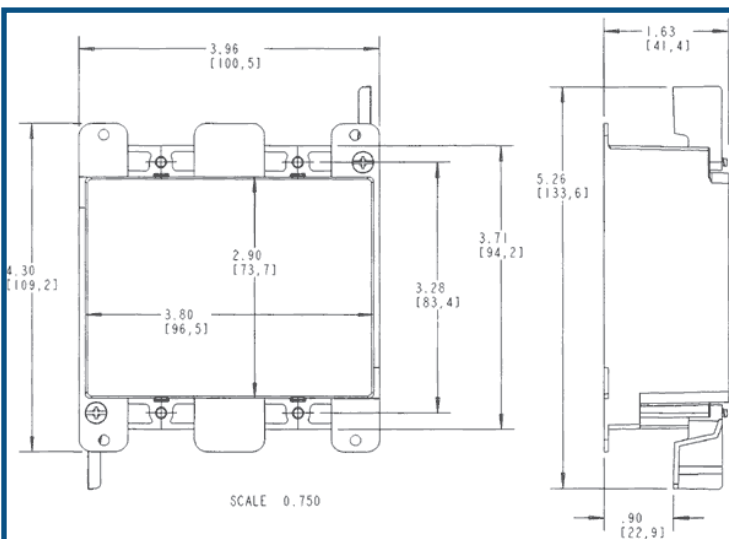
2-GANG EXSISTING CONSTRUCTION ^
