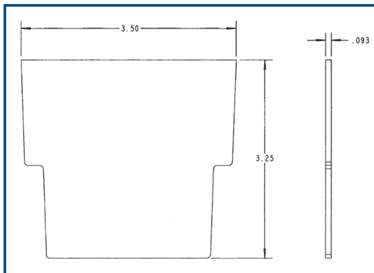
LOW VOLTAGE DIVIDER PLATE
