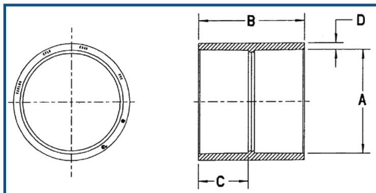
STANDARD COUPLING
