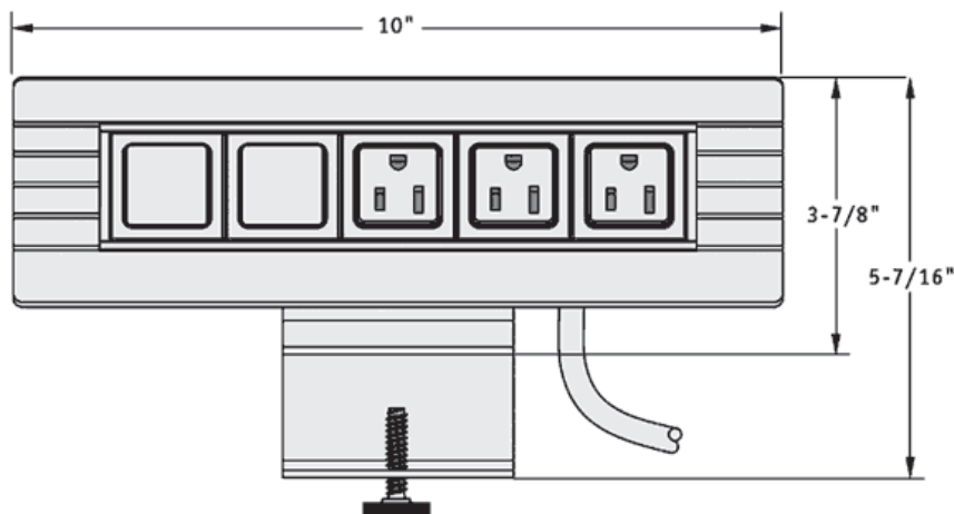
Front Dimensions
