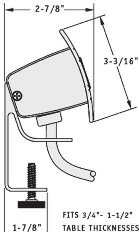
Side Dimensions
